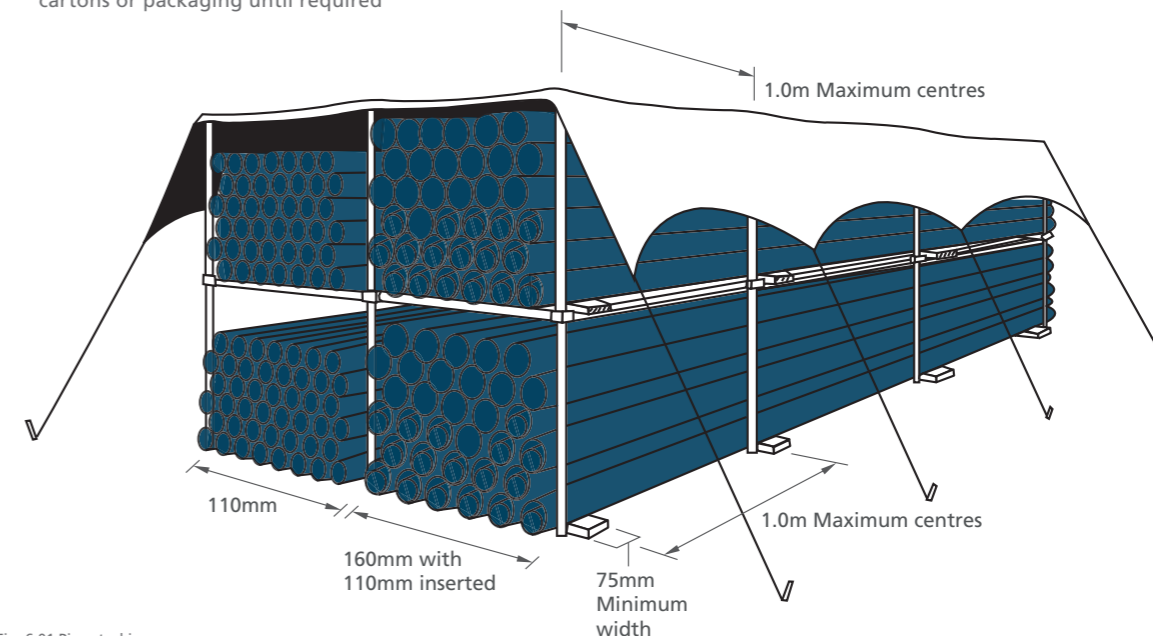
Fig. 6.01 Pipe stacking
