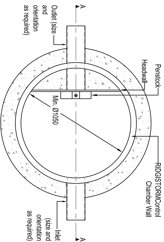
PLAN VIEW Scale (1:30)
