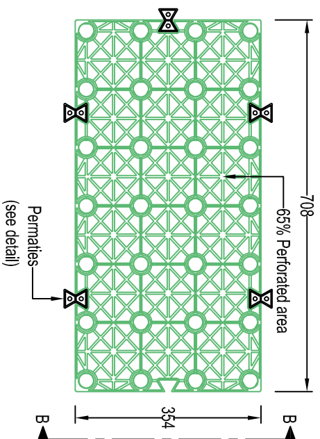
PLAN Scale (1:10)
