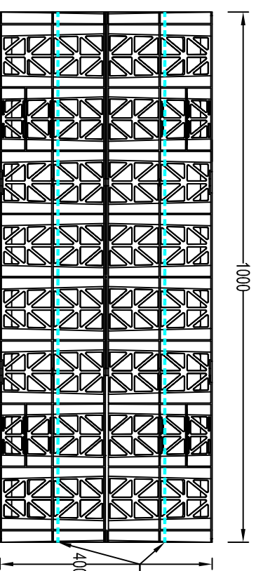
ELEVATION A-A Scale (1:10)
