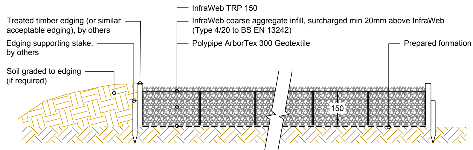
TYPICAL SECTION Scale 1:10
