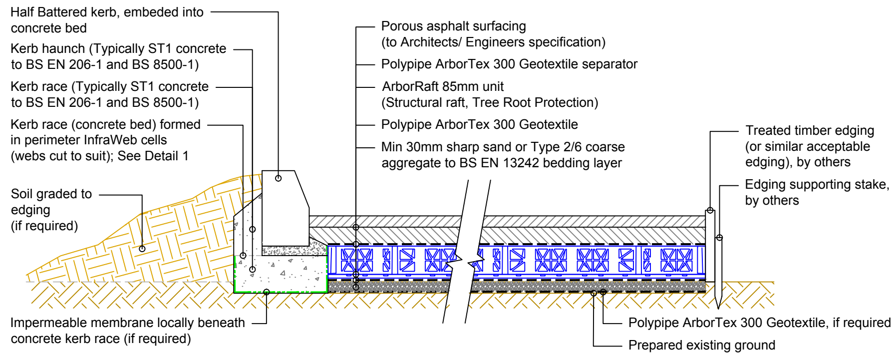
TYPICAL SECTION Scale 1:10
