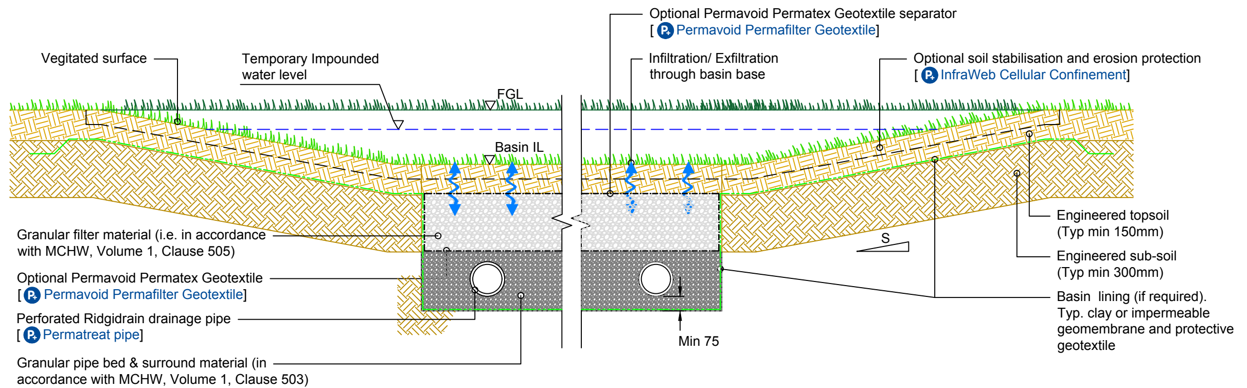
TYPICAL SECTION
