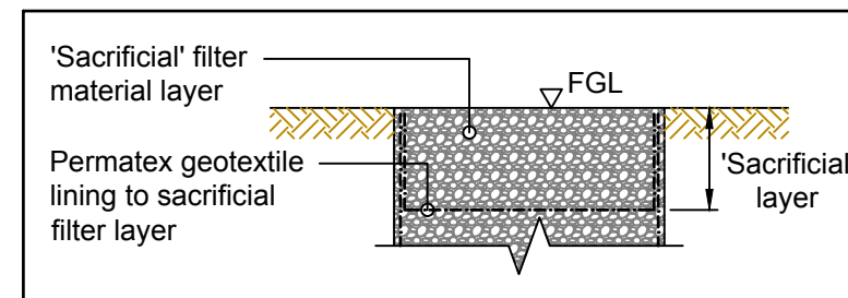
Optional Surface Detail - Sacrificial Surface Layer
