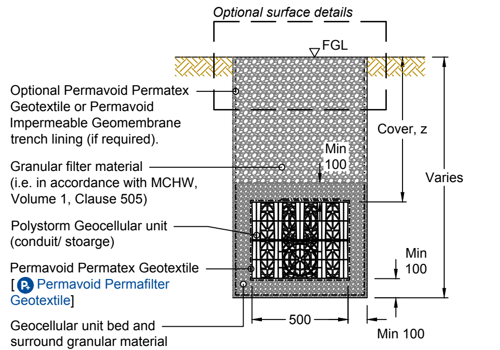
TYPICAL SECTION
