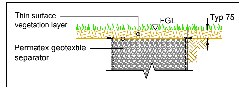
Optional Surface Detail - Vegetated Surface
